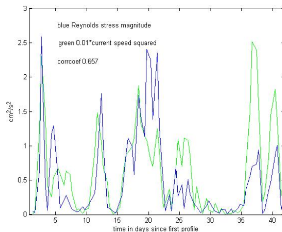
Fig. 6. Magnitude of Reynolds Stress and 0.01 * \text{Current Speed Squared} .
