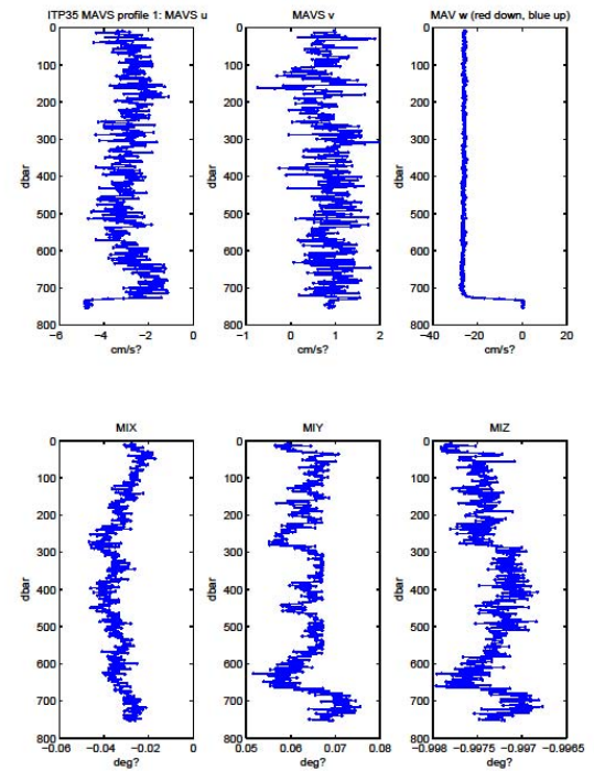
Fig. 8. MAVS data from the first up profile of the ITP under the ice. The top row shows velocity into the sensor, velocity across the sensor and vertical velocity. The lower row shows three components of earth magnetic field direction cosines.
